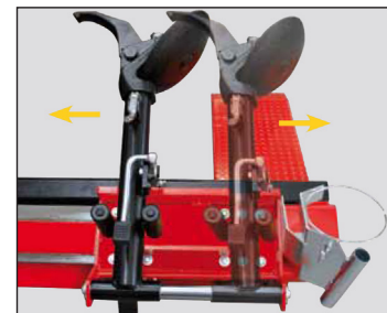
Carriage with hydraulic left/right translation and tool arm with safety lock system.
